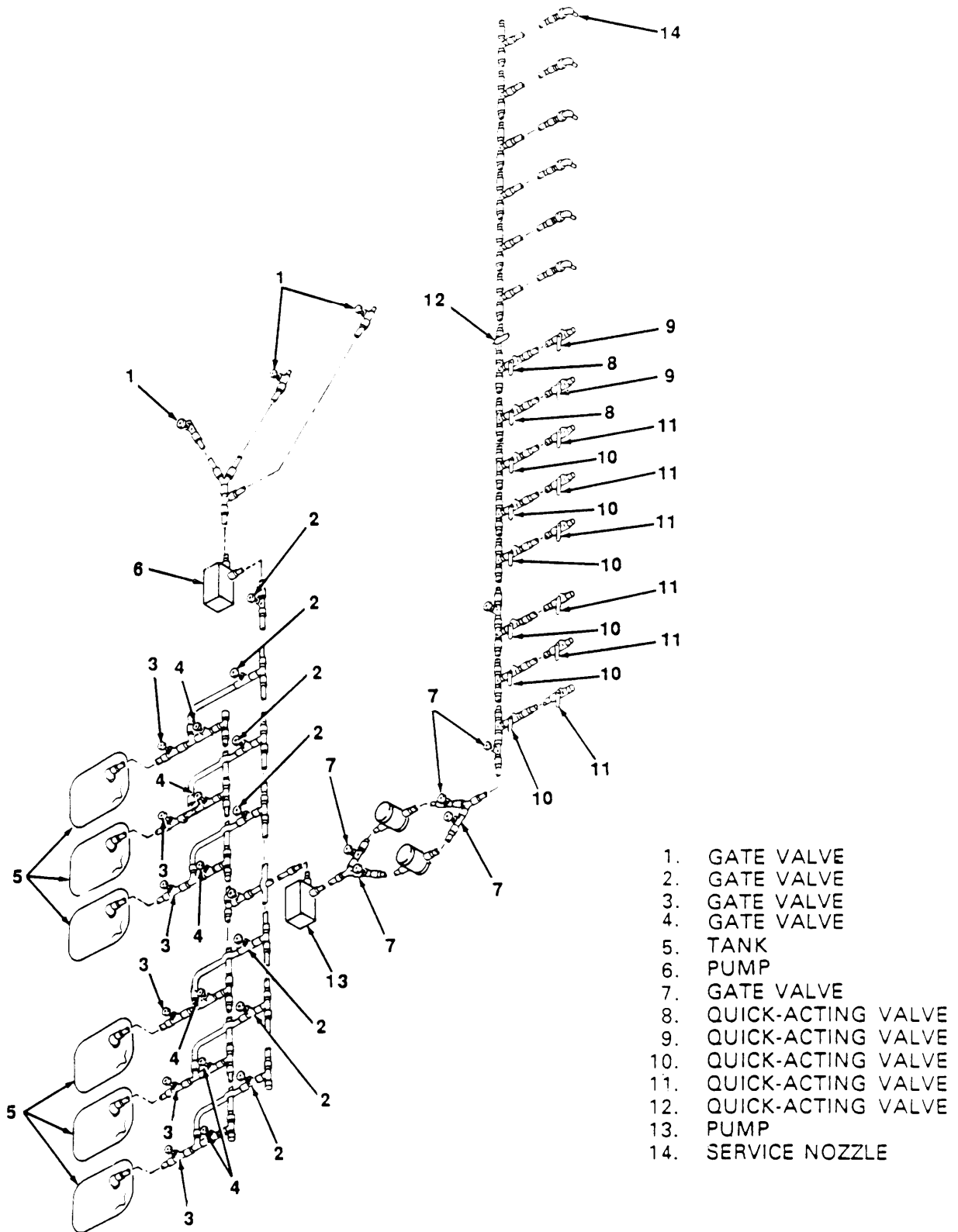
Figure 2-2. Fuel System Operation.
