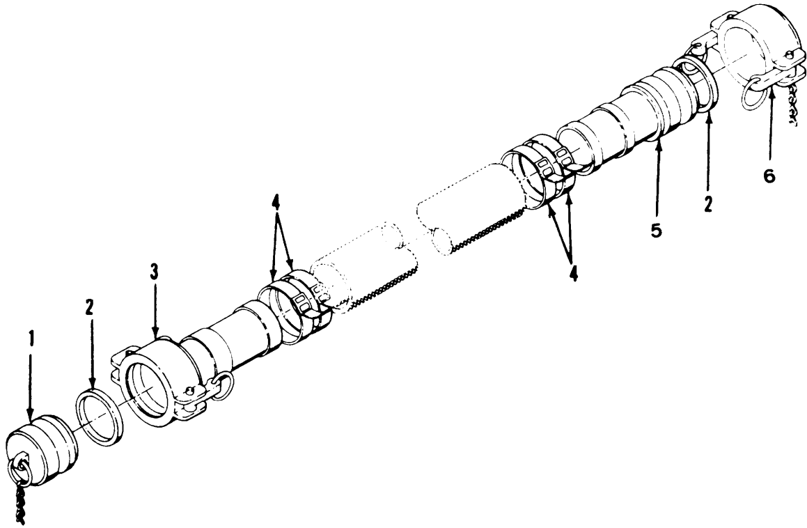
Figure F-9. Discharge Hose Assembly, 3 In. X 25 Ft.
