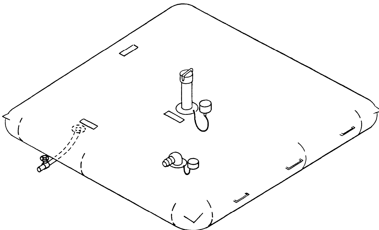
Figure 1-5. Collapsible Storage Tank, 10,000 Gallons.
